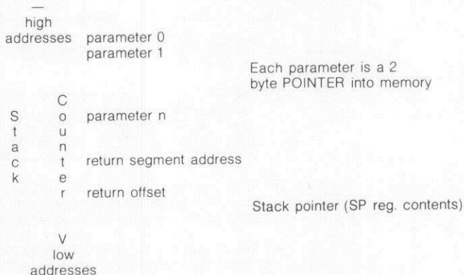
Figure E-1: Stack Layout when CALL Statement is Activated
